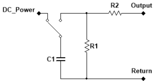
Figure 1 Power Line Waveform Circuit Schematic
