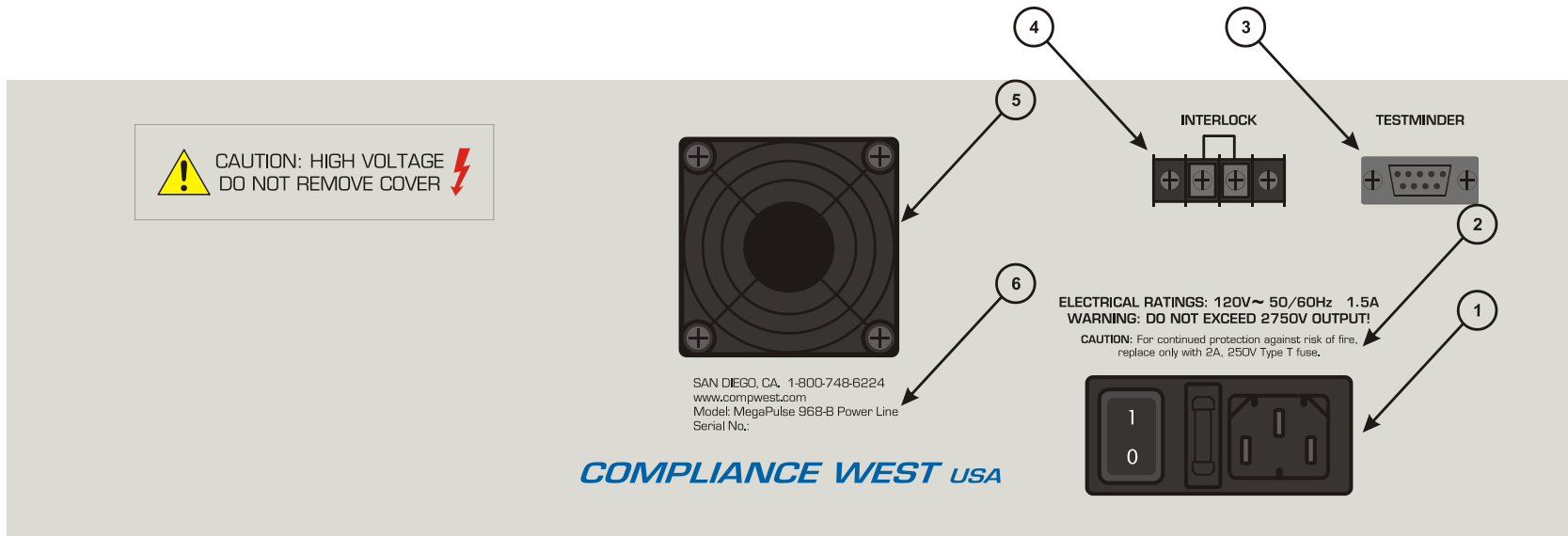
Figure 3 MegaPulse 968-B Power Line Rear Panel
