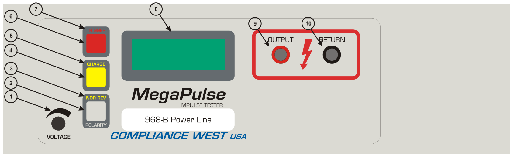
Figure 2 MegaPulse 968-B Power Line Front Panel
